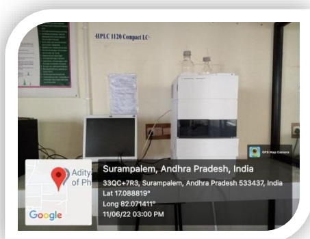
HPLC
